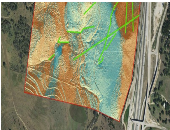
Linear features identified from slope aspect investigations.
